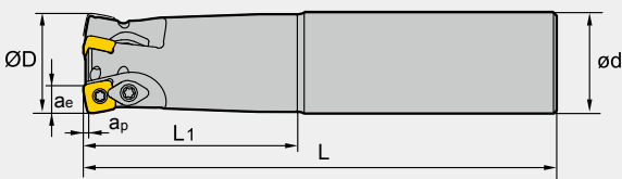
S type insert straight shank type
