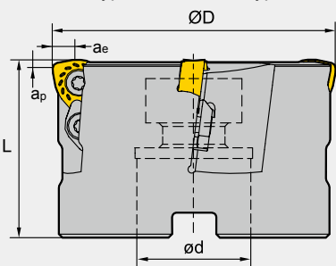
W type insert sleeve type
