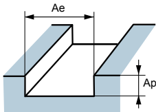
FigureA Milling groove
