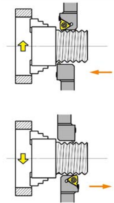
External processing Left hand thread
