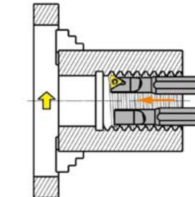
Internal processing Left hand thread
