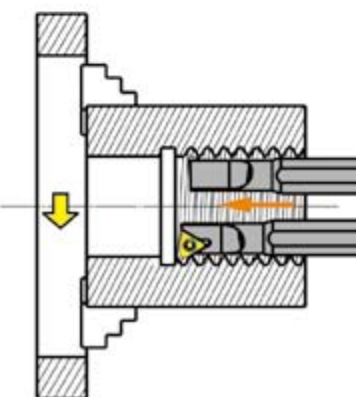
Internal processing Right hand thread
