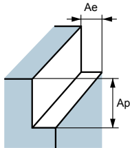
FigureB Square shoulder milling
